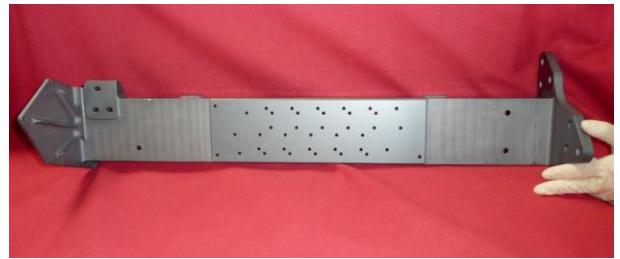
Fig. 9. The VNIR detector support (3.6 kg)
