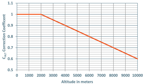
Graph 4: Altitude derating
