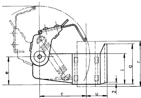
Type BZ
