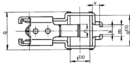
Type BZ
